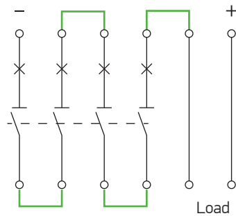
DC MCCB (1000 V - 4P)
