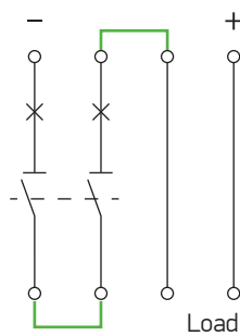
DC Fuse 2P (SDC10000 - 500 V)
